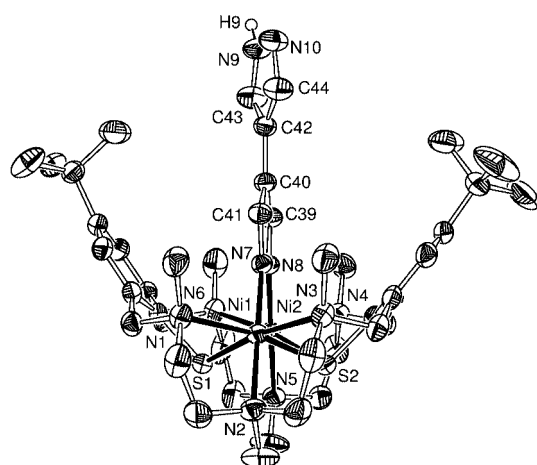
Figure 1. ORTEP representation of the structure of the [L^1Ni^{II}_2(Hbpz)]^+ cation in crystals of 6[BPh_4] \cdot 1.5MeCN . Ellipsoids are represented at the 50% probability level. Hydrogen atoms except H(9) have been omitted for clarity.
