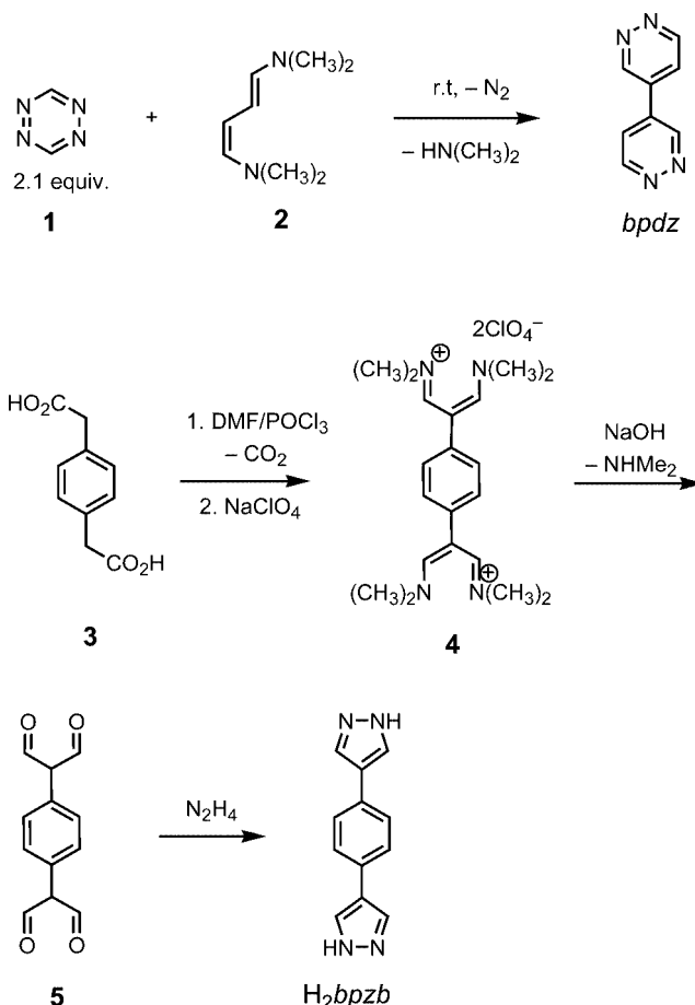
Scheme 2. Synthesis of the heterocycles \text{H}_2\text{bpzb} and \text{bpdz} .
