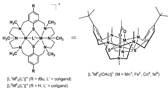
Scheme 1. Dinuclear complexes of the hexaaza-dithiophenolate ligands (L^1)^{2-} and (L^2)^{2-} .
