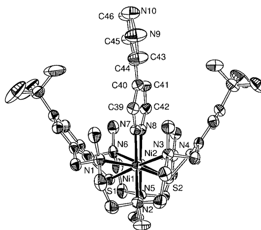
Figure 2. Structure of the [L^1Ni^{II}_2(bpdz)]^{2+} dication in crystals of 7[ClO_4]_2 \cdot 3MeCN with thermal ellipsoids at the 50% probability level. Hydrogen atoms are omitted for reasons clarity.
