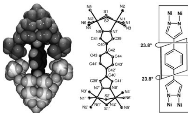
Figure 3. Left: Van der Waals plot of the [(\text{L}^1\text{Ni}^{\text{II}}_2)_2(\text{bpzb})]^{2+} dication in crystals of 8 [\text{BPh}_4]_2 \cdot 6\text{MeCN} \cdot 2\text{H}_2\text{O} . Middle: ORTEP representation of the core structure of 8 with the atom labeling Scheme. Ellipsoids are represented at the 50% probability level. Symmetry code used to generate equivalent atoms: 1 - x, 1 - y, 1 - z ( ' ). Right: Mutual orientation of the \text{Ni}_2\text{pyrazolato} planes in 8 .
